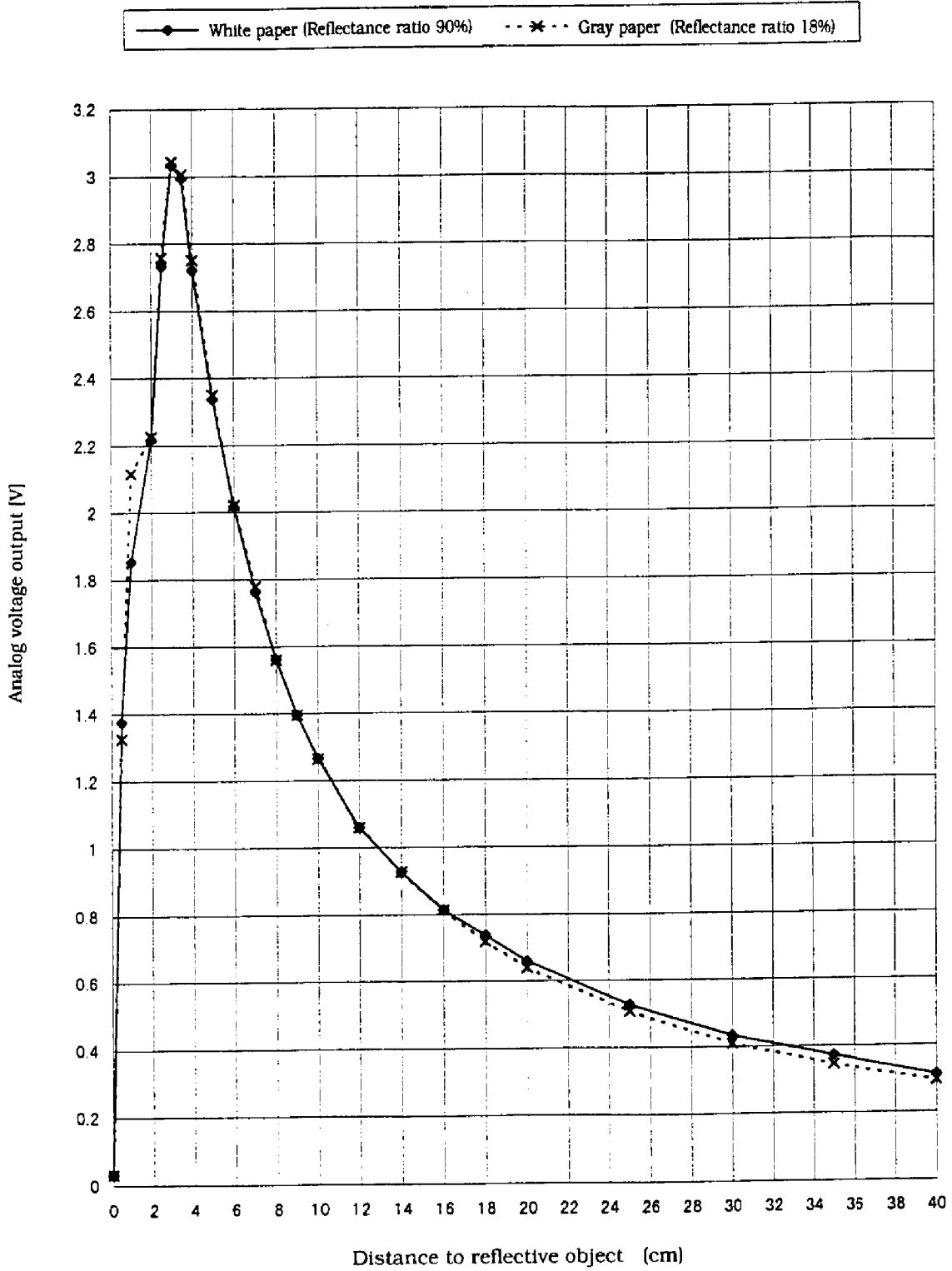
6-1 GP2D120 Example of Output distance characteristics
