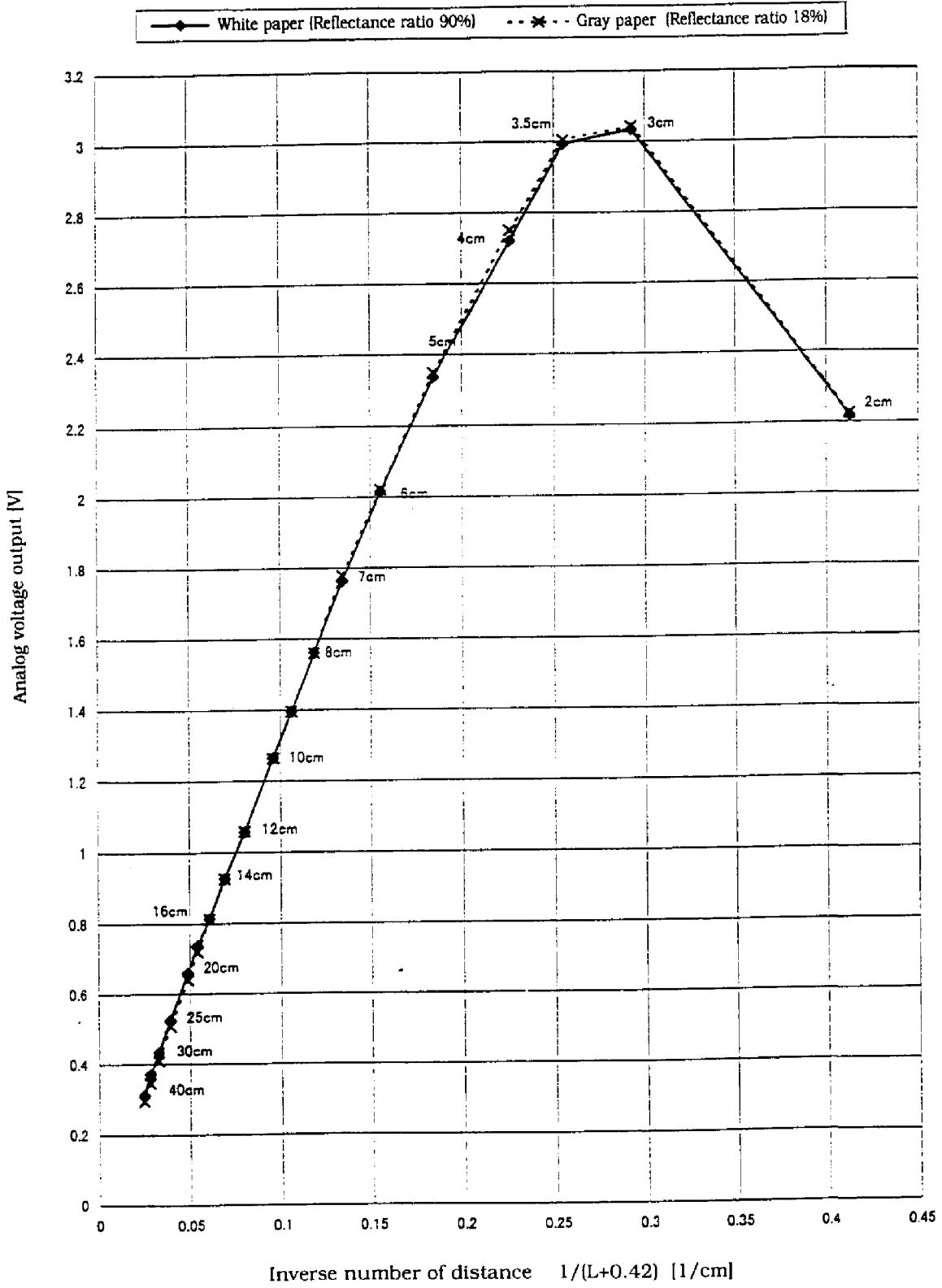
6-2 GP2D120 Example of output characteristics with inverse number of distance
